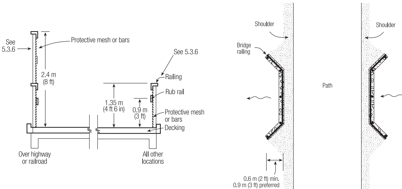
Figure 5-8. Bridge Railings.
