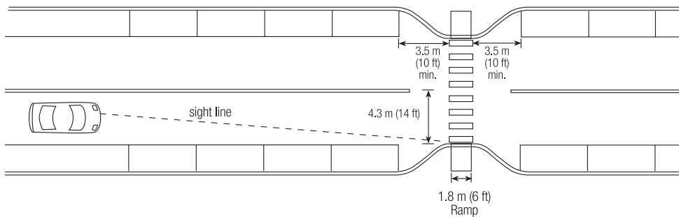
Figure 3-42. Typical Curb Extension Design at a Mid-Block Crossing
