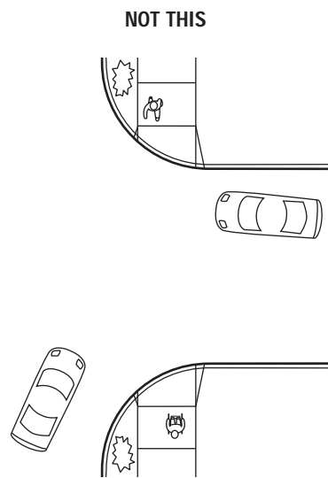
Figure 3-15. Intersection-Style Driveway May Encourage High-Speed Turns
