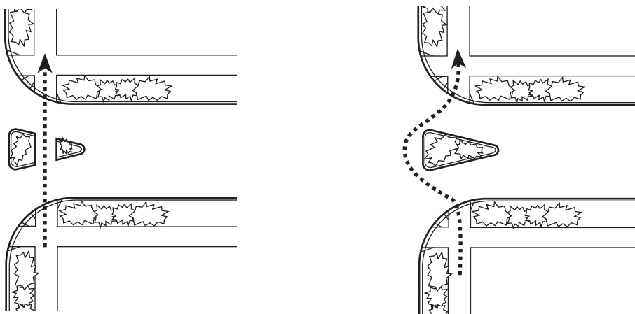
Figure 7-8. Maintain Walkway Continuity at Splitter Islands
