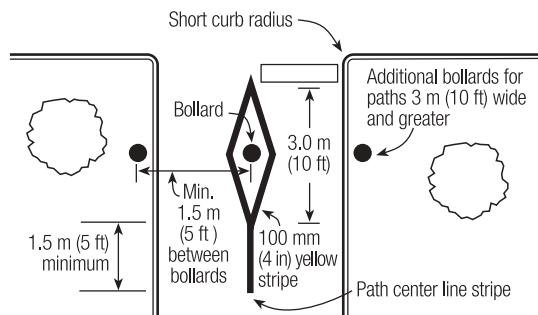
Figure 5-15. Bollards.
