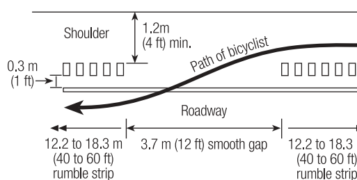
Figure 4-27. Rumble Strips.
