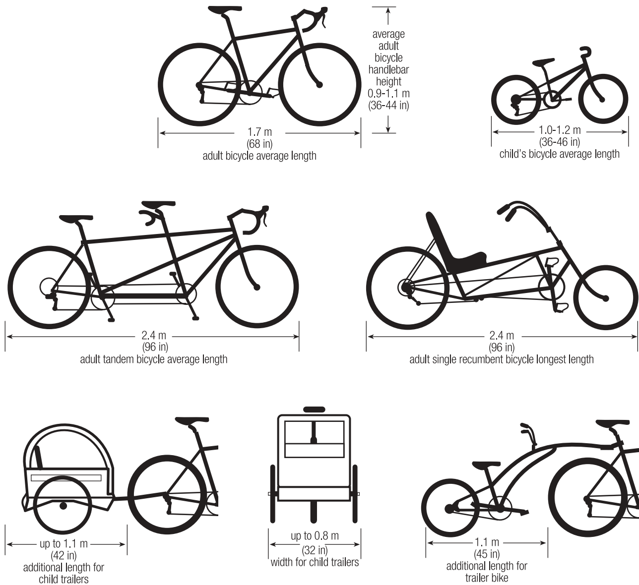
Figure 4-1. Bicycle Styles and Dimensions.
