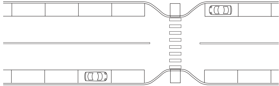
Figure 7-3. Curb Extensions.
