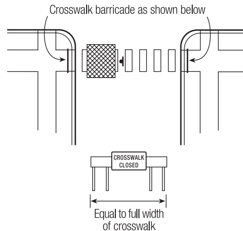
Figure 8-5. Crosswalk Closure
