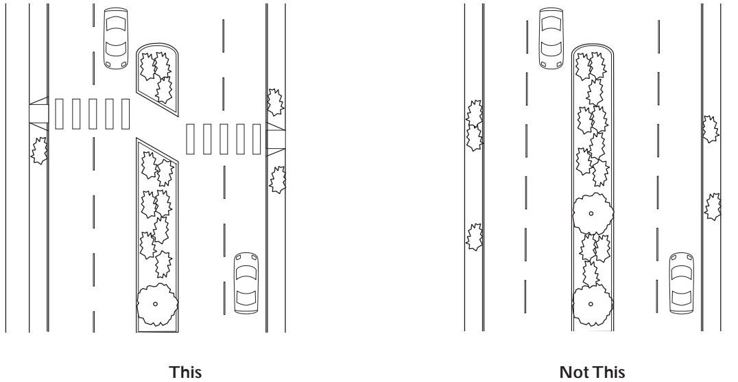
Figure 7-11. Ensure Access at Medians.
