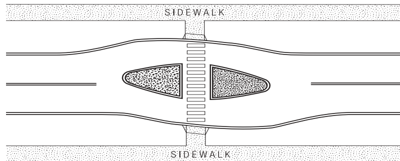
Figure 7-5. Raised Median.
