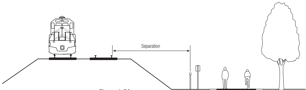
Figure 6-7A. Separation, Rails-With-Trails.
