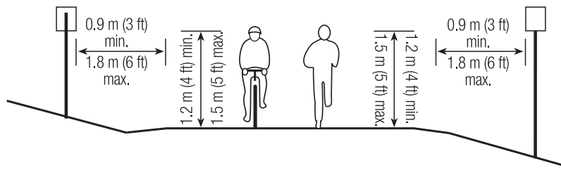
Figure 8-18. Sign Placement on Shared Use Paths.
