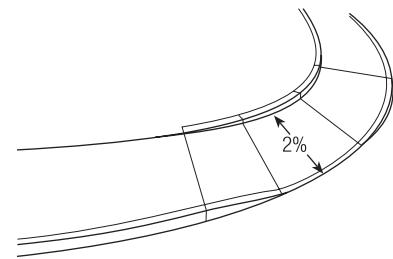
Figure 3-28. Diagonal Variation
