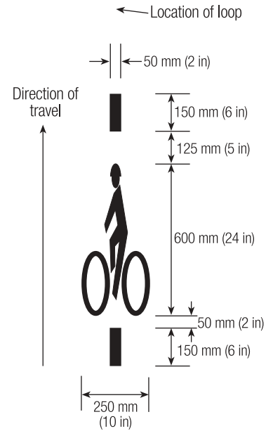
Figure 8-17. Pavement Marking to Identify a Bicycle Sensitive Location.
