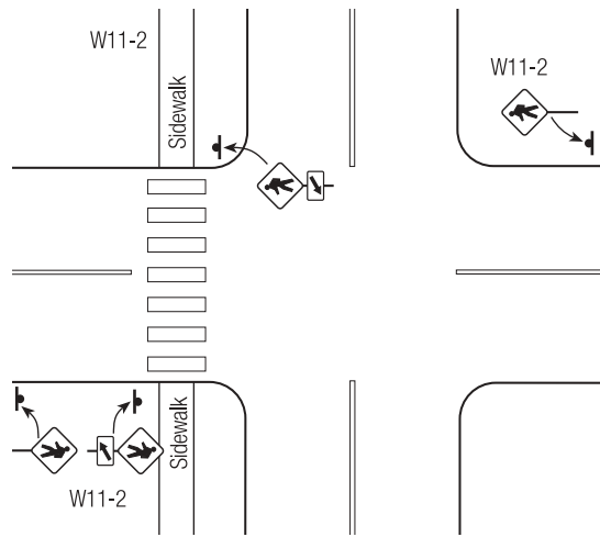
Figure 3-41. Uncontrolled Approach to an Intersection
