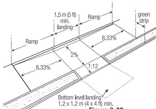
Figure 3-29. Combination Curb Ramp, Midblock Location
