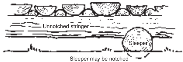
Figure 47—Rustic tread or decking made from half logs (logs cut in half lengthwise).
