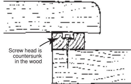
Countersinking
