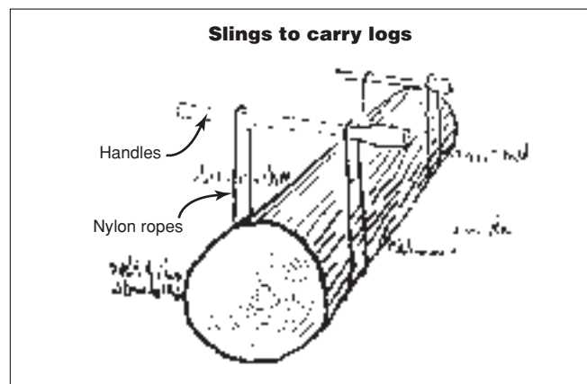
Figure 92—Slings are a good way to move logs and timbers, bundles of steel bars, wheelbarrows that must be carried over soft ground, or bags of cement carried on plywood.
