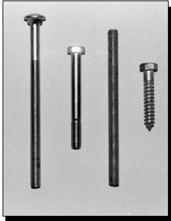
Figure 69—Fasteners (from left): carriage bolt, machine bolt, all-thread rod, and lag screw.
